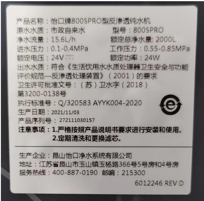
800SPRO (铭牌)
